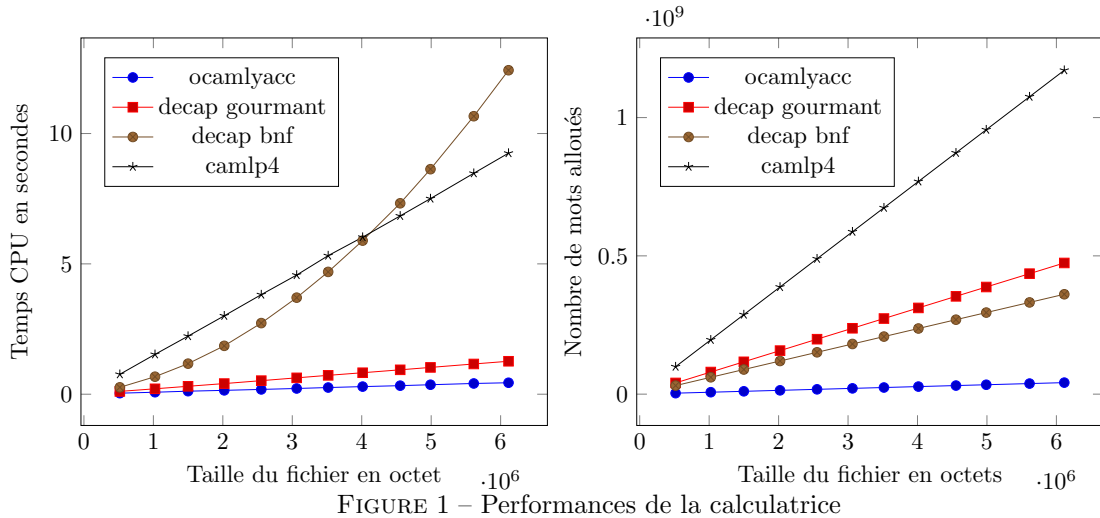
FIGURE 1 – Performances de la calculatrice
